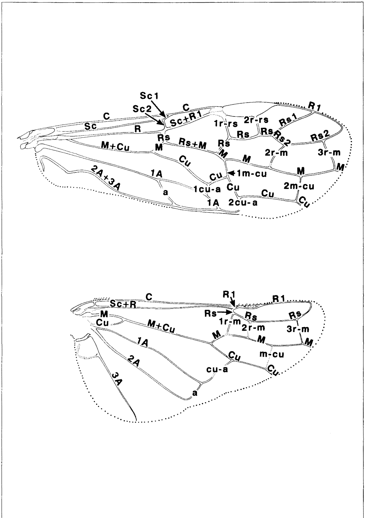
Fig. 15. Wing veins of Macroxyela sp. (Symphyta: Xyelidae).
