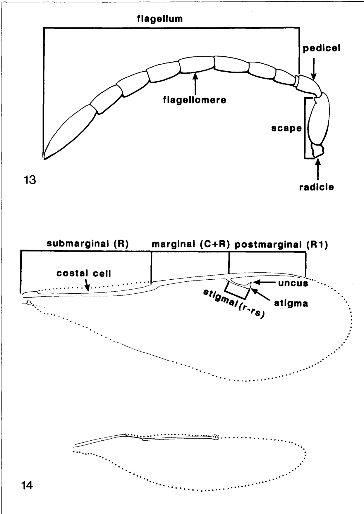
Fig. 13. Antenna of Macroneura sp. (Apocrita: Eupelmidae). Fig. 14. Fore and hind wings of a pteromalid (Apocrita: Chalcidoidea).
