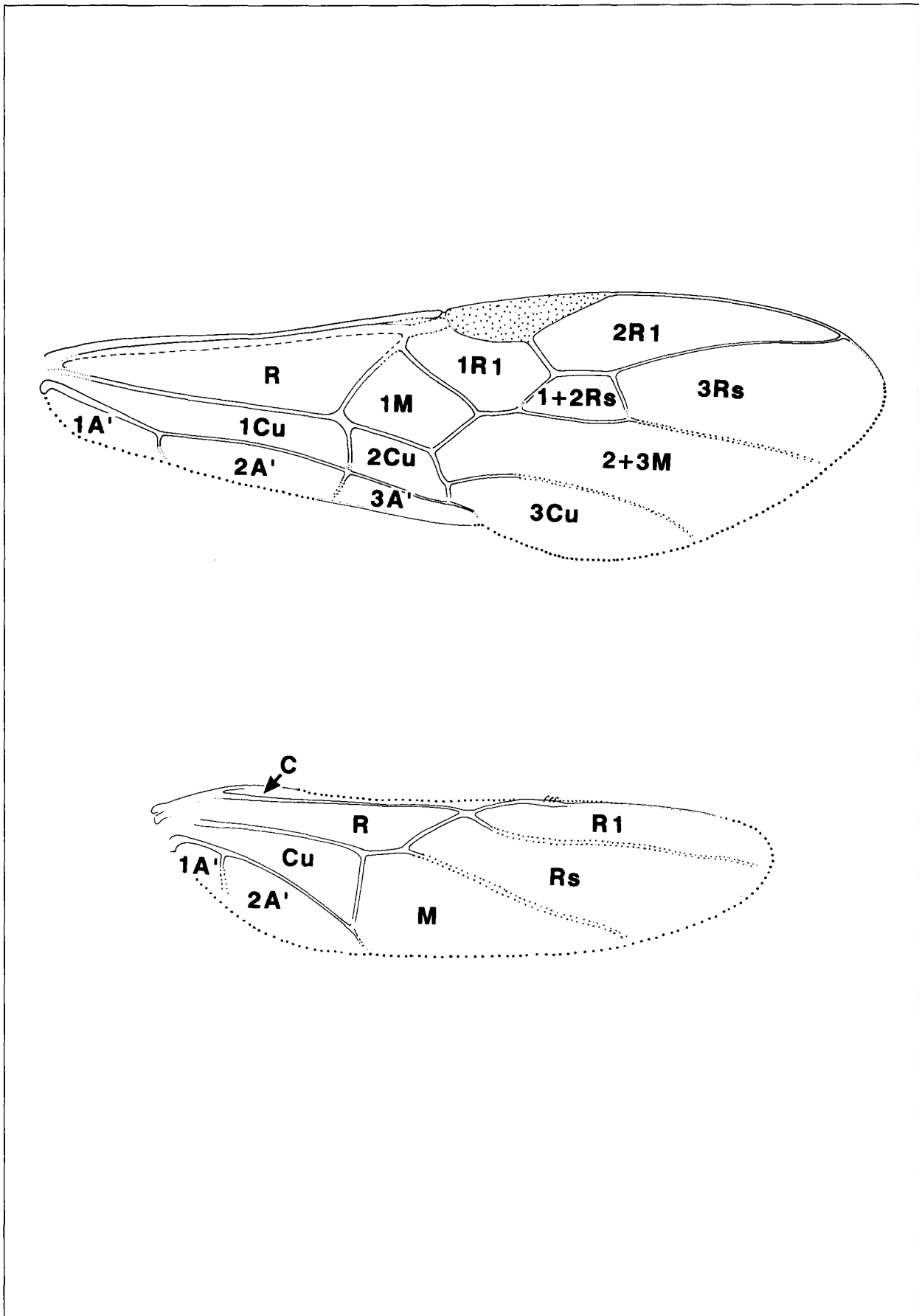
Fig. 18. Wing cells of Helcon sp. (Apocrita: Braconidae). Cell names given with Fig. 16.
