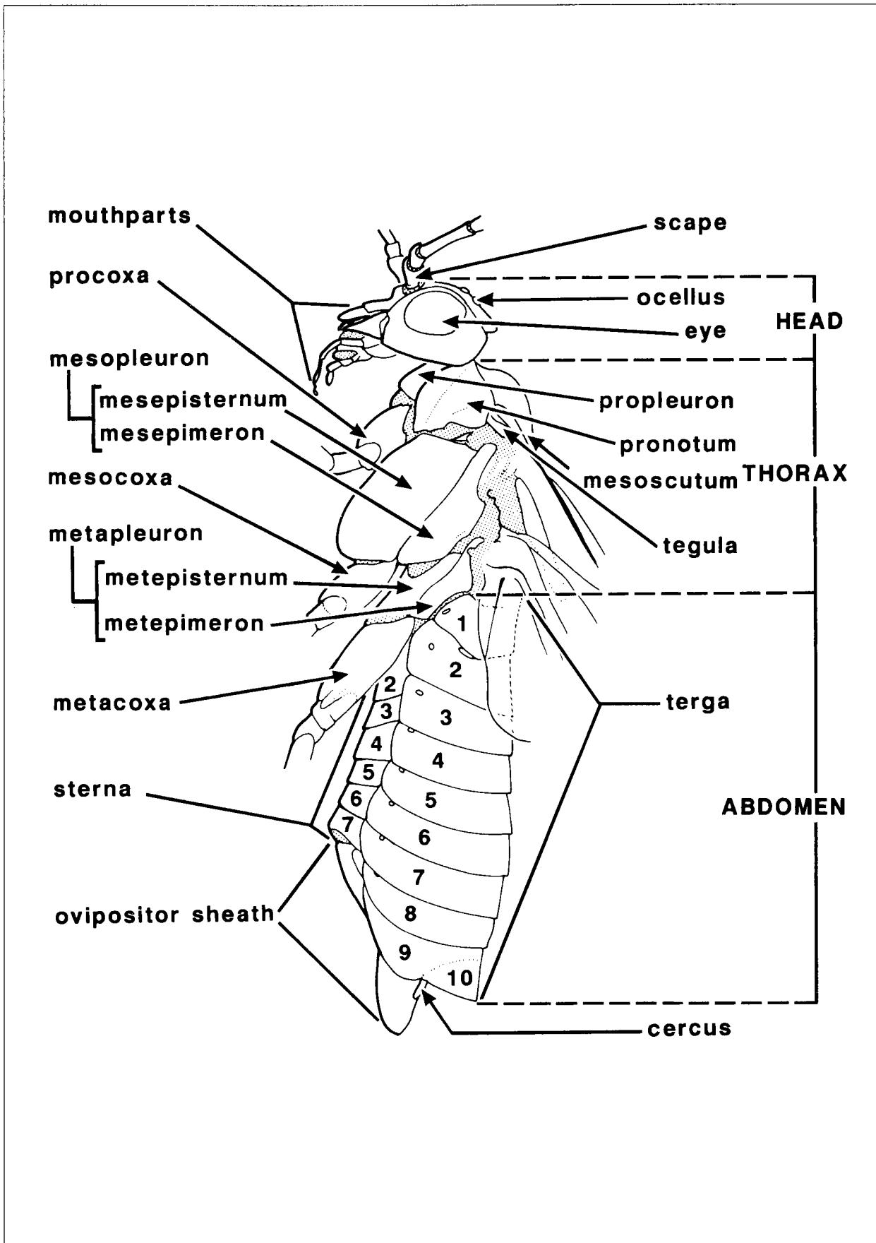
Fig. 3. Main morphological divisions and structures of a species of Symphyta, Aglaostigma quattuordecimpunctatum (Norton) (Tenthredinidae): lateral view.
