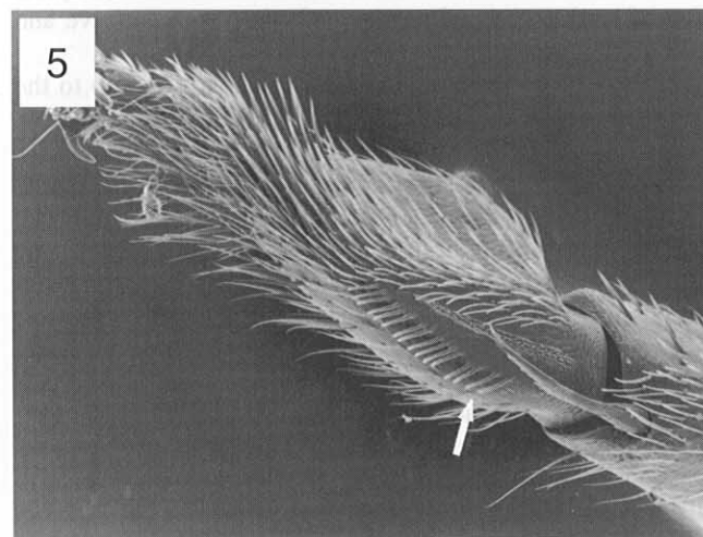
Figures 1–6. Scanning electron micrographs of M. emeryi showing silk producing spinnerets, protarsal silk brush and mesotarsus. 1. Ventral view of head showing buccal cavity and mandibles. Arrows indicate hairs along margin of buccal cavity and tuft of hair on mandible; scale = 100 \mu\text{m} . 2. Silk producing glands on the external cuticular surface of the margin of the buccal cavity, showing slits in the cuticular margin where silk fibers originate (arrow); scale = 10 \mu\text{m} . 3. Enlarge-
