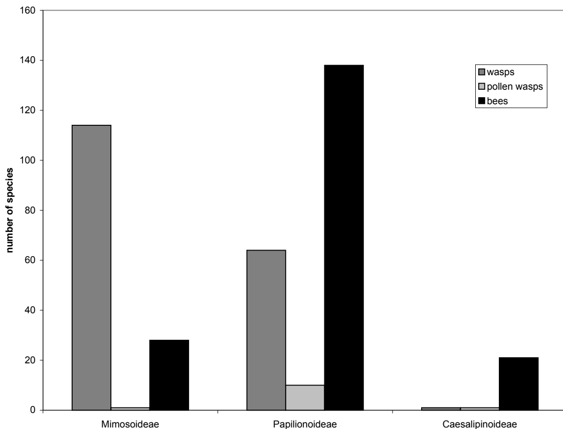
Fig. 19. Comparison of the complexes of wasps, pollen wasps and bees visiting the three subfamilies of Fabaceae.
